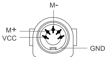
5-pin connector (pinout: C-DIN-51R)
