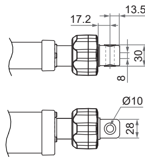
Solid type Zinc alloy with MR3 (For Push load only) 7: Solid with bushing, Ø10mm 8: Solid w/o bushing, Ø12mm
