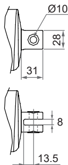
Slot type Zinc alloy, 90° pivot 5: Slot with bushing, Ø10mm 6: Slot w/o bushing, Ø12mm
